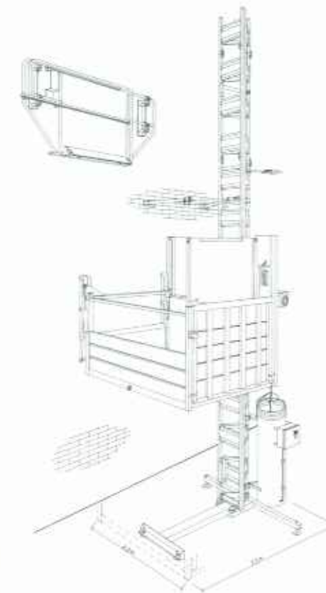
Hot-dip galvanised landing level safety gates (1 piece is supplied with the base unit) with mechanically locked sliding door are installed at the landing levels to ensure safety of people.
